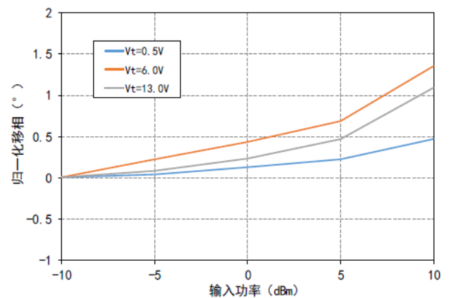
归一化移相VS Pin@10GHz
